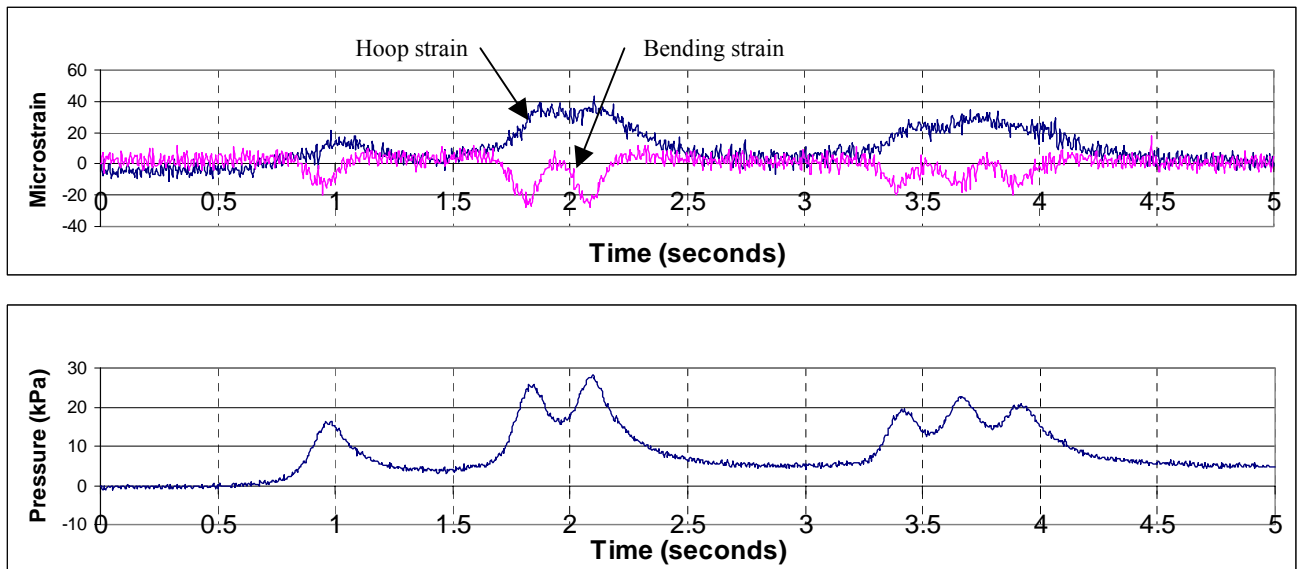
Figure 10: Plot of Hoop and Bending Strain and Pressure at Top of Culvert
