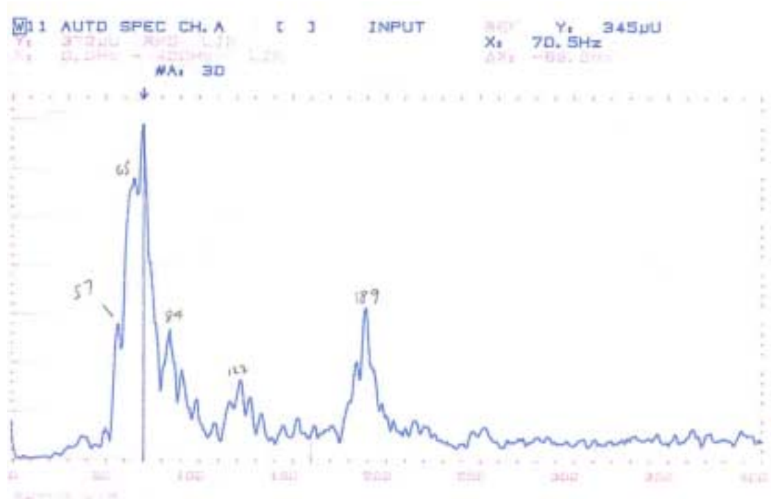
Figure 5: Transverse Beam Vibration Spectrum – Anzac Bridge
