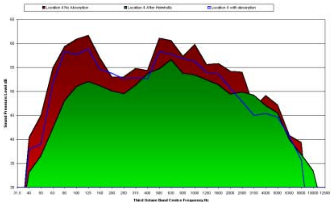
Figure 6: RMS Average Third Octave Band Noise Spectra at Location 4
