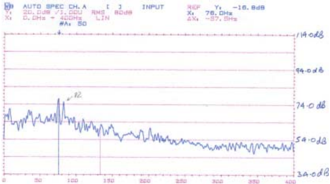
Figure 4: Acoustic Excitation Spectrum – Tom Ugly’s Bridge
