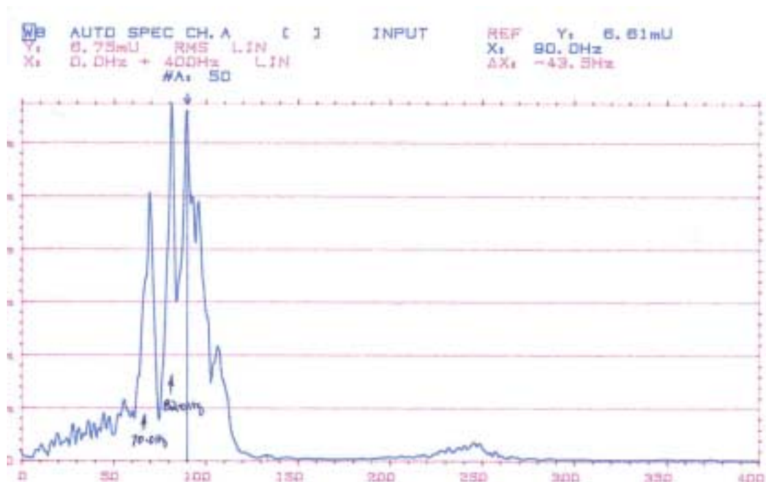
Figure 3: Transverse Beam Vibration Spectrum – Tom Ugly's Bridge
